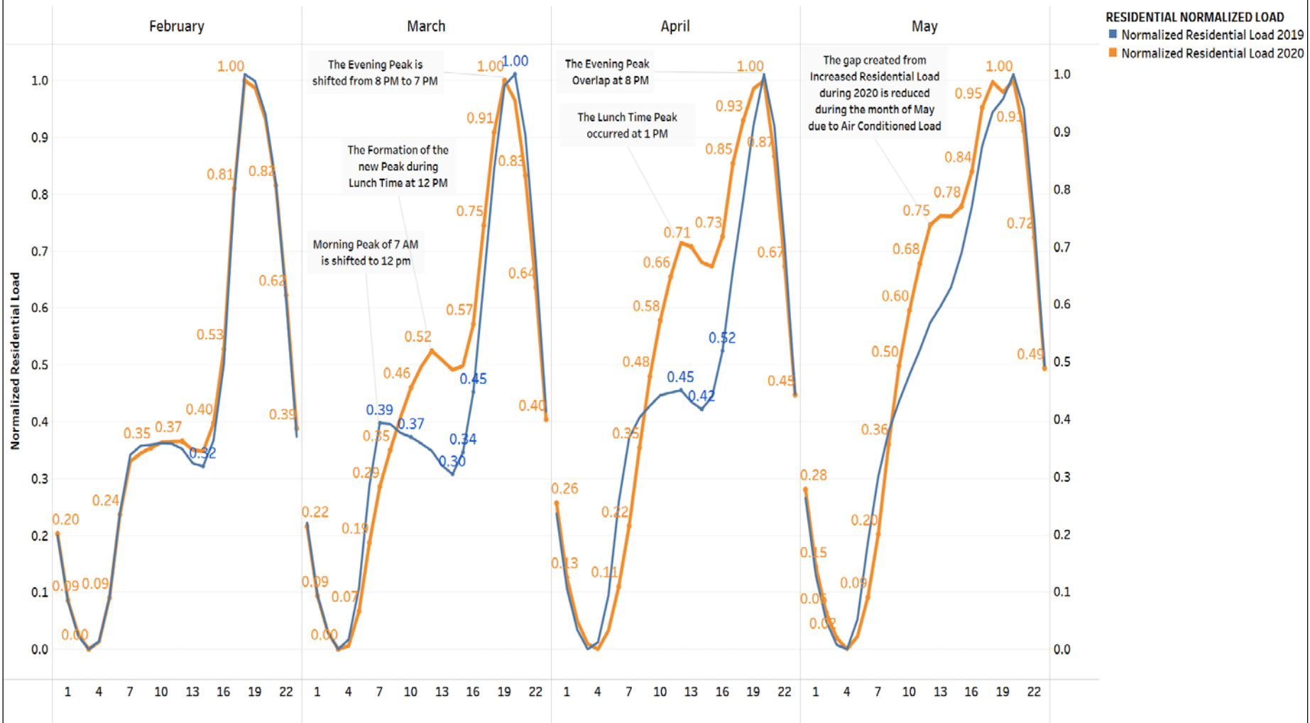
Residential Normalized Monthly Hourly Average Load
