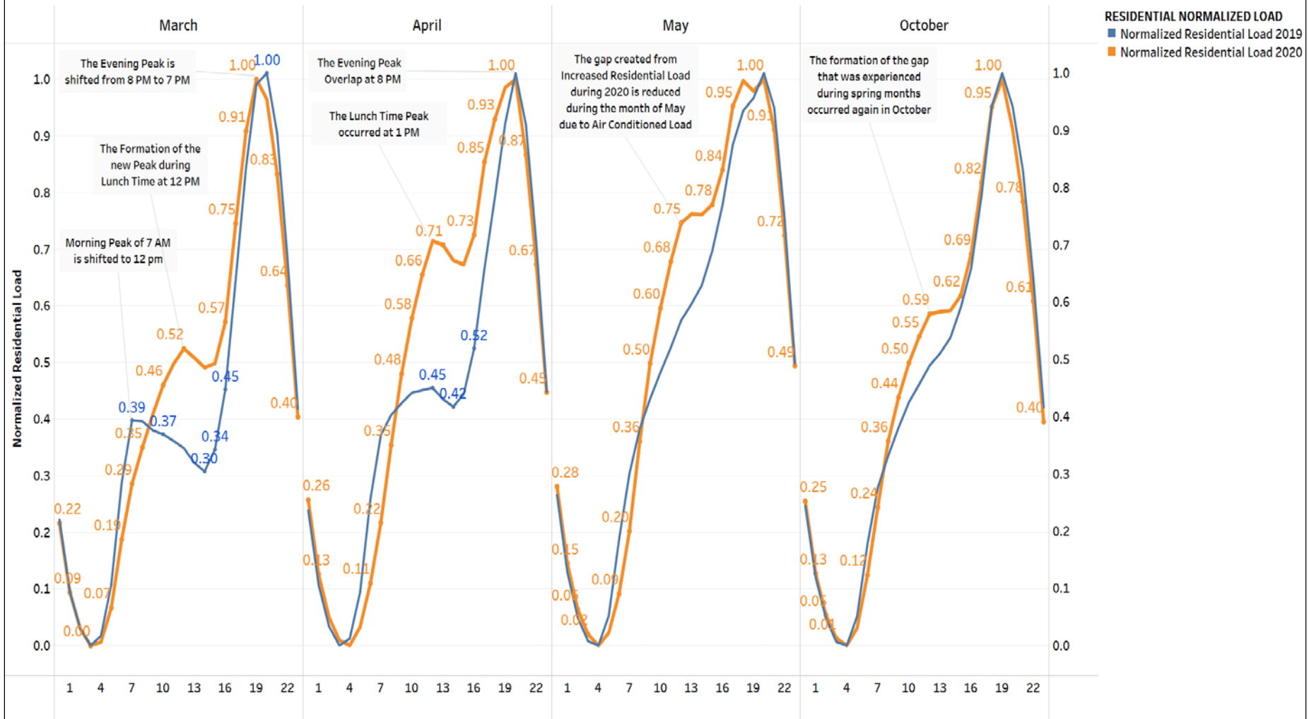
Residential Normalized Monthly Average Load
